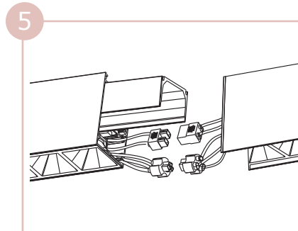
5. Connect with same colour wires
