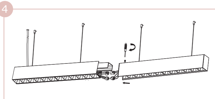
4. Connect wires from each LED module
