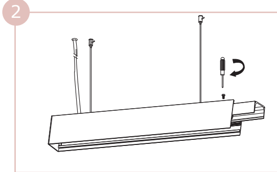
2. Fix the connecting piece on the first fixture
